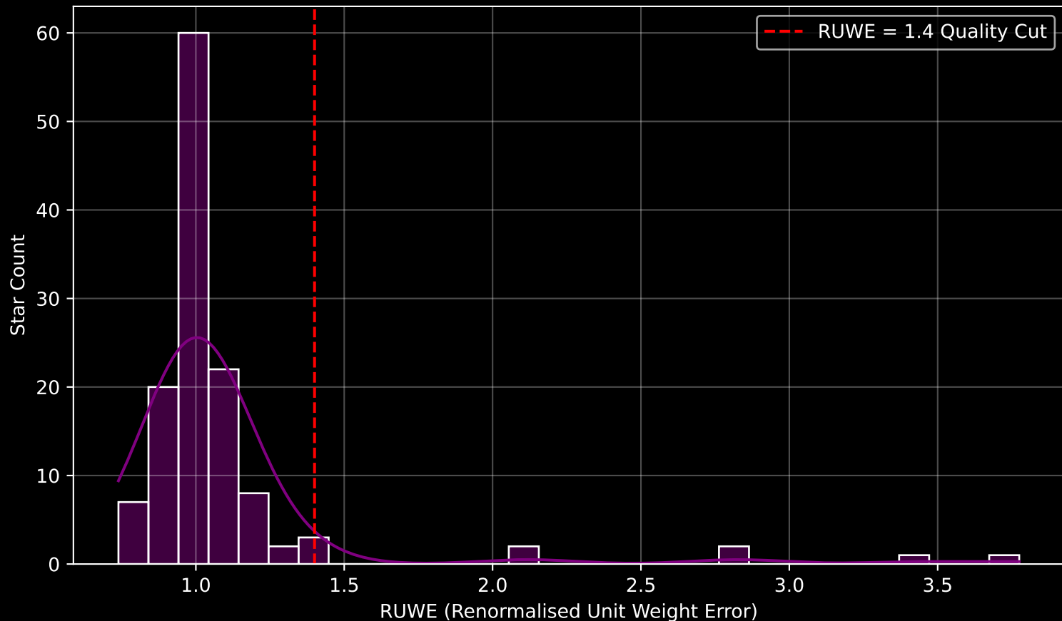
GAPOGEE DR17 Field [SGRCMI+02] RUWE Distribution (n= 128)
