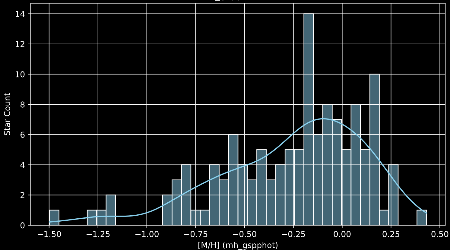
APOGEE DR17 Field: [SGRCMI+02 [M/H] (mh_gspphot) (n= 127)
