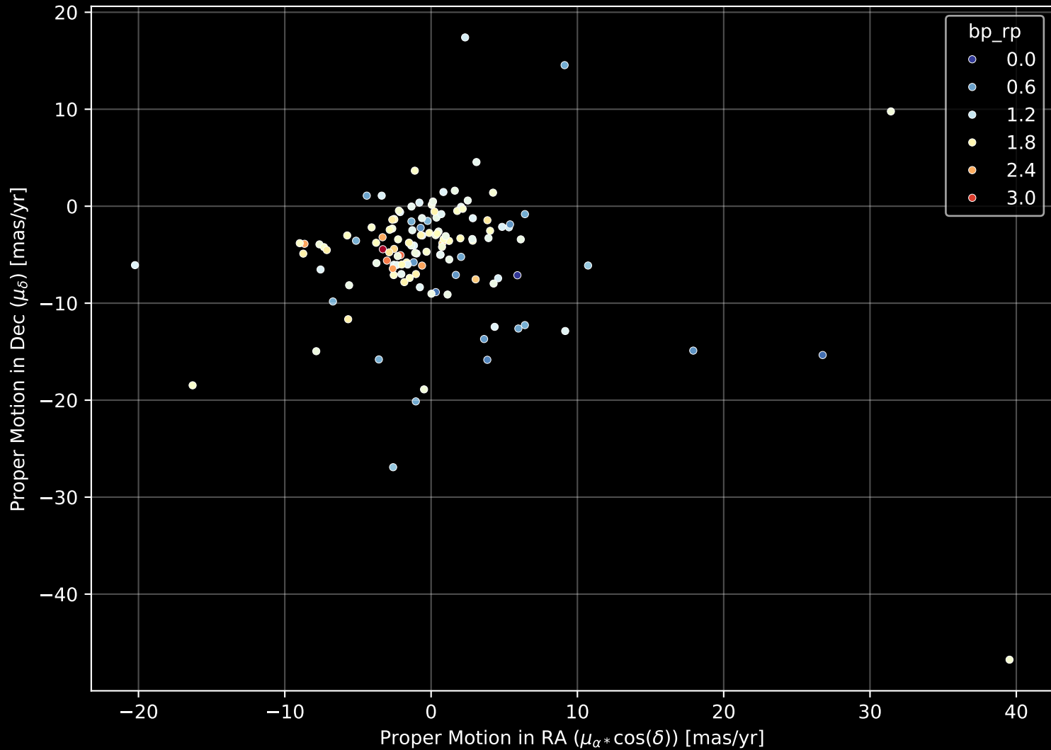
APOGEE DR17 Field: [SGRCMI+02] Proper Motion Diagram (n= 129)
