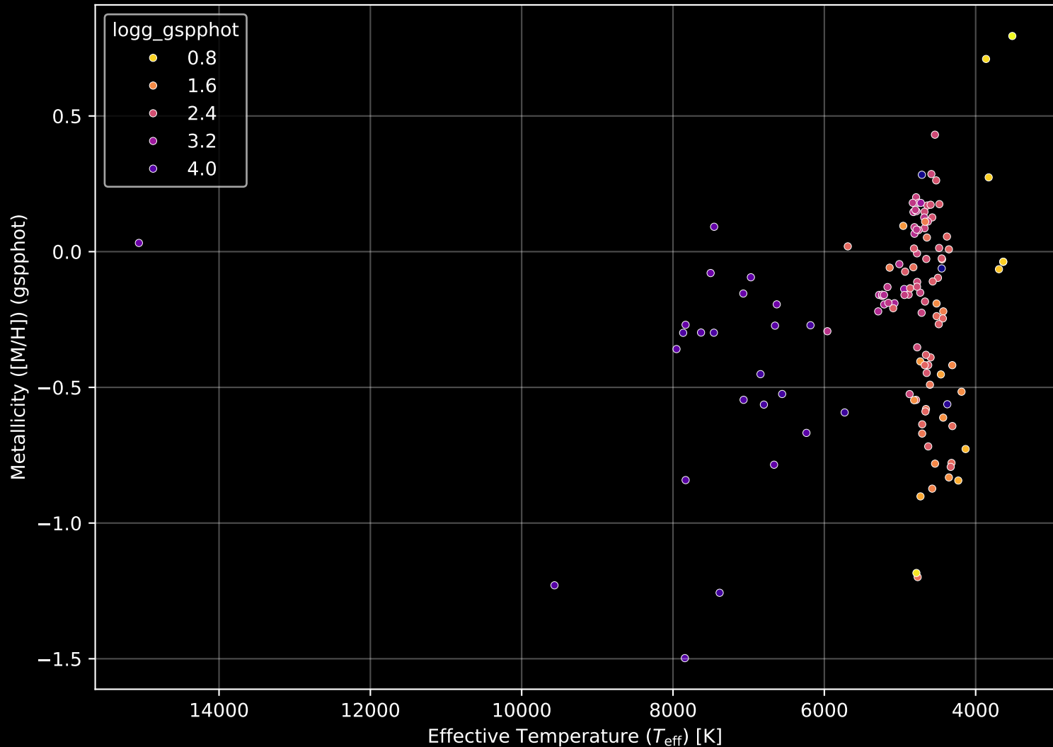
APOGEE DR17 Field: [SGRCMI+02] Stellar Population Parameters (n= 129)
