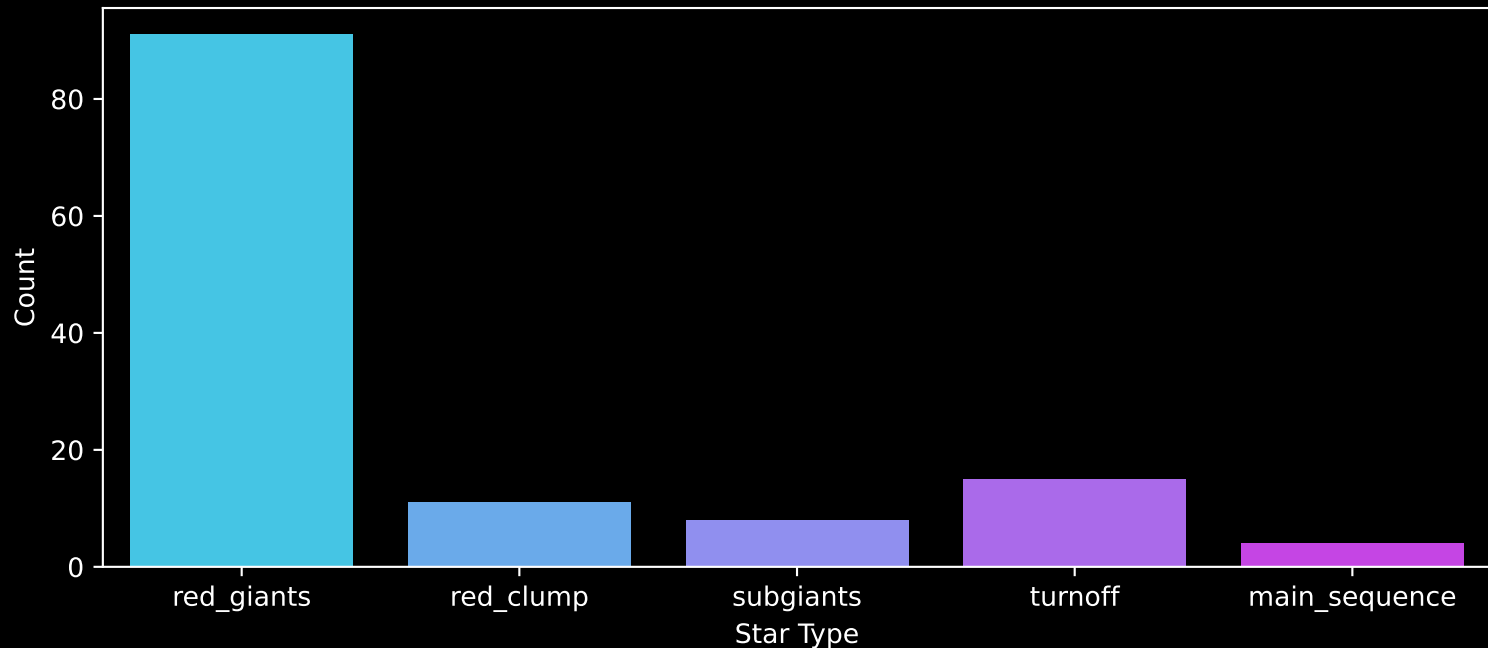
APOGEE DR17 Field: [SGRCMI+02] Count plot of Star Type
