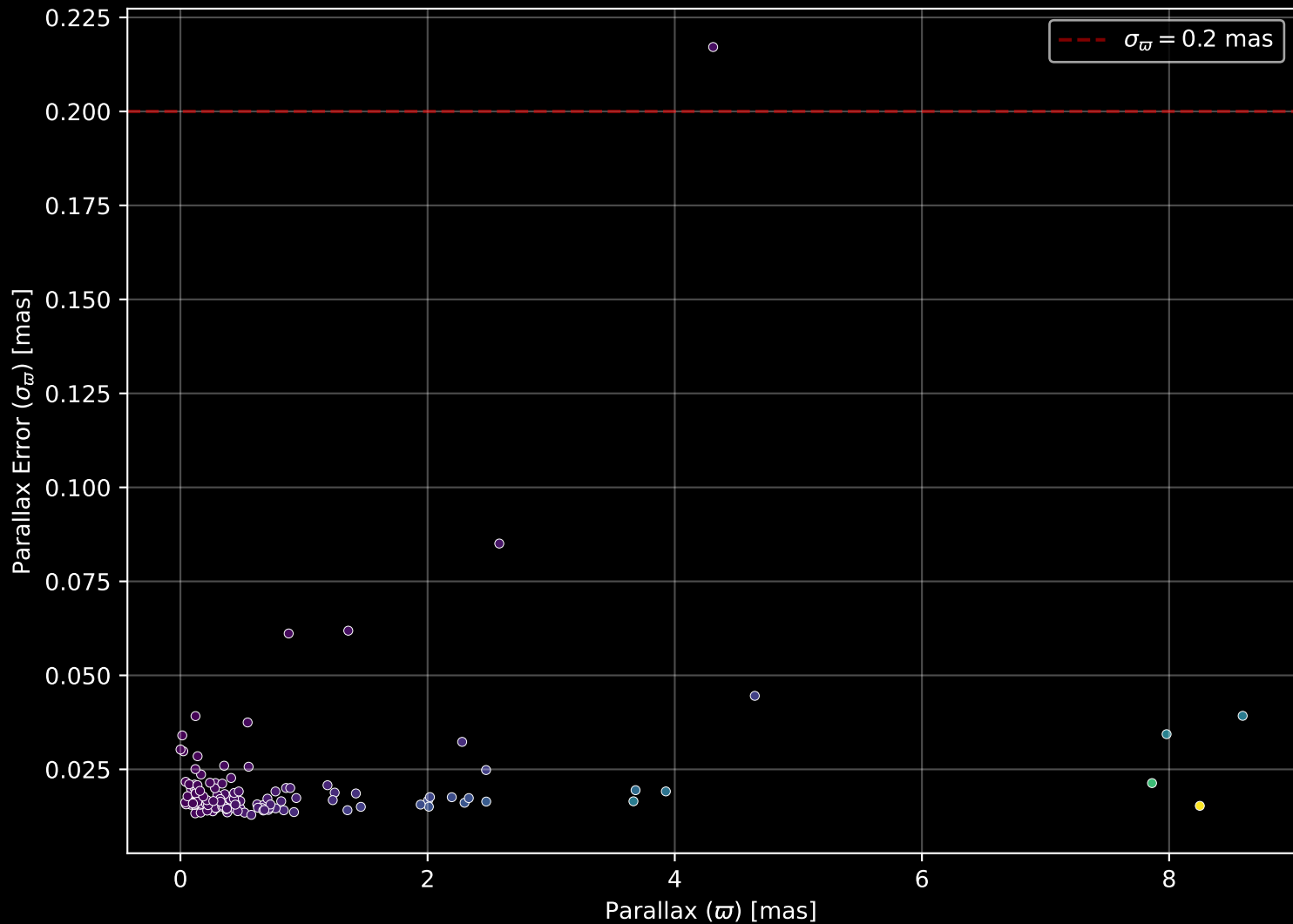
APOGEE DR17 Field: [SGRCMI+02] Parallax Quality (n= 129)
